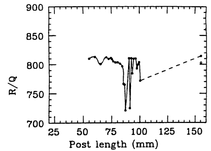
Fig. 12 Measured R/Q (MΩ/m) vs. post length.
