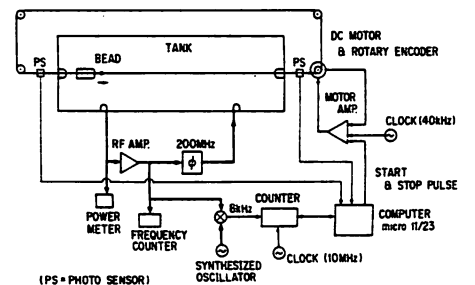
Fig. 3 Block diagram of the field measurement.
