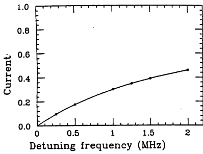
Fig. 4 Calculated sum of post currents at the stabilization when perturbation is given to the both end cells.
