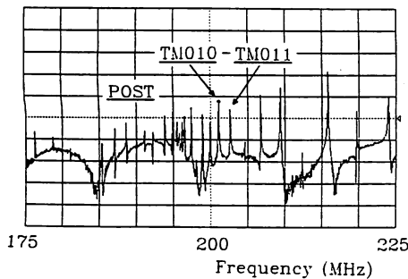
Fig. 7 Measured resonant modes at the stabilization.
