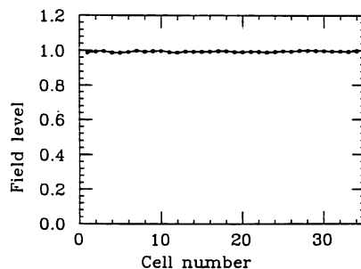
Fig. 8 Measured TM010 field at the stabilization.
