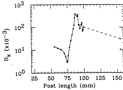
Fig. 11 Measured distortion parameter vs. post length.
