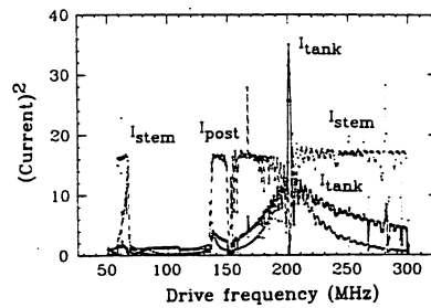
Fig. 14 Calculated modes at the stabilization. \omega_2 = 142.4 MHz.
