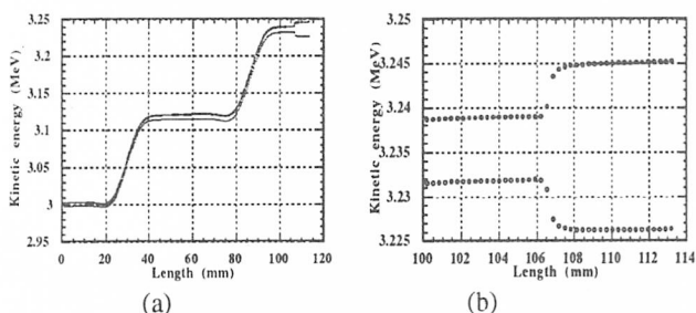
Fig.5 (a) Longitudinal energy variation through the initial two cells for two particles. A change in the energy due to a collision can be seen at a length of 107 mm. (b) A magnified plot of (a).
