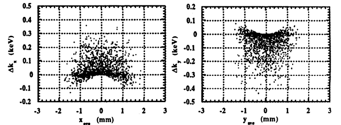
Fig. 3 Change in the transverse kinetic energies through the cell vs. the average transverse coordinates when the magnetic gradient is turned on.
