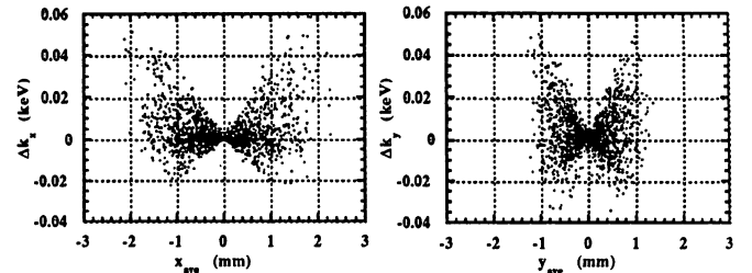
Fig. 2 Change in the transverse energies through the cell vs. the average transverse coordinates for both transverse directions ( B'=0 ).
