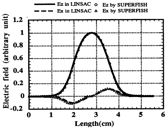
Fig. 1 Field distributions in the unit cell used in the LINSAC code.
