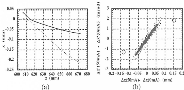
Fig.4 (a) Trajectories ( x vs. z ) of two collision particles through the eleventh cell. (b) Difference between the change in the x -gradient for a 50-mA beam within the eleventh cell and that for a 0-mA beam as a function of the difference in corresponding x -coordinates. The two circles indicate the collision particles.
