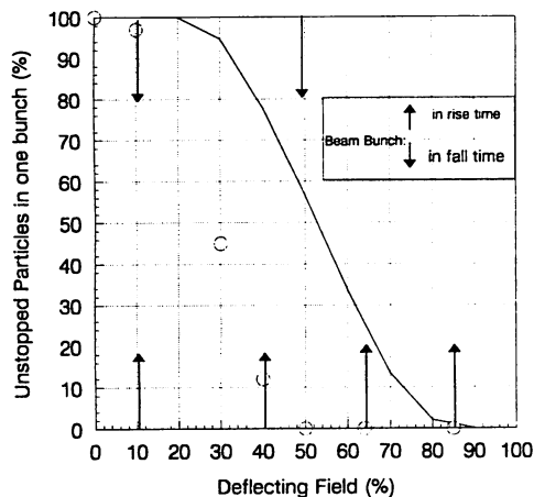
Fig.3 Unstopped particles ratio in one bunch vs the deflecting field variation. The arrows indicate the bunch distribution during the RF rising and falling time. The line indicates at the entrance of DTL and the circles the exit of DTL.
