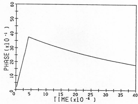
Fig.11 Calculated phase shift at z=L/2 due to beam loading.
