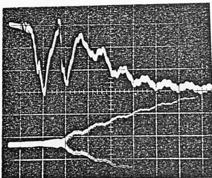
Fig. 2 Transient phase shift between z=L and master oscillator (one feed).
