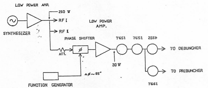
Fig.15 Blockdiagram of phase compensation of debuncher.
