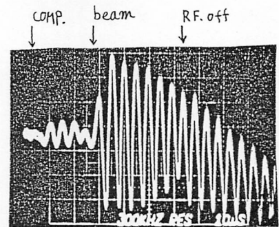
Fig.13 Beat frequency.
