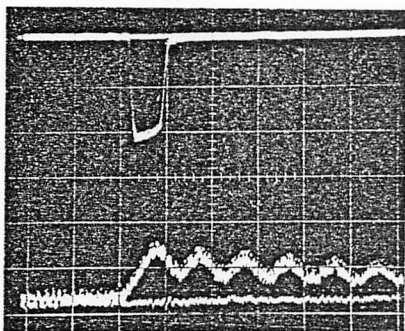
Fig. 6 Transient phase shift due to beam loading between z=L and master oscillator. Upper trace is linac beam pulse (~140mA).
