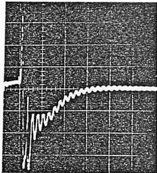
Fig. 4 Transient phase shift between z=0.3L and z=L (one feed).
