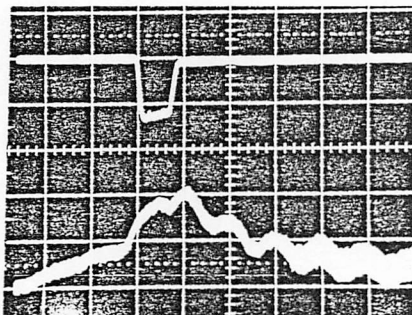
Fig. 8 Transient phase shift due to amplitude compensation and beam loading measured at z=0.2L .
