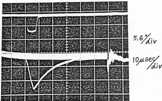
Fig.14 Phase shift of debuncher rf field due to beam loading.
