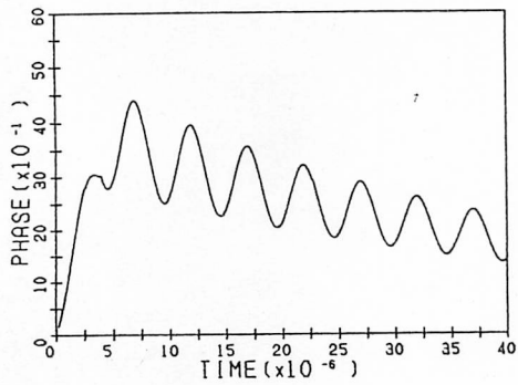
Fig.10 Calculated phase shift at z=L due to beam loading.
