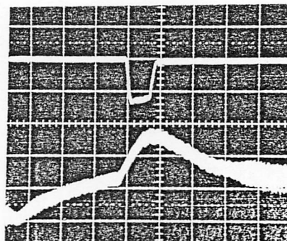
Fig. 9 Transient phase shift due to amplitude compensation and beam loading measured at center of tank.
