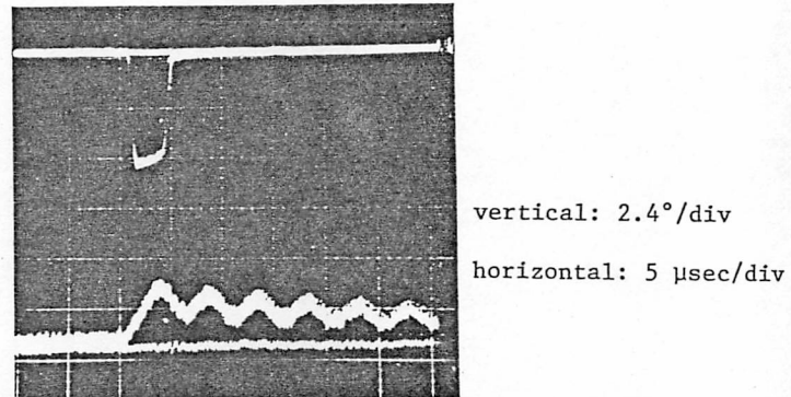
Fig. 5 Phase shift due to beam loading measured at z=0.9L . Upper trace is the output beam.
