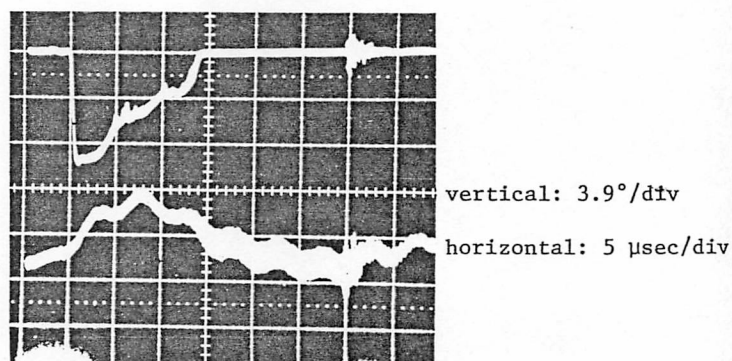
Fig. 8 Phase shift due to the beam of 15 \mu\text{sec} . Upper trace shows the output beam.
