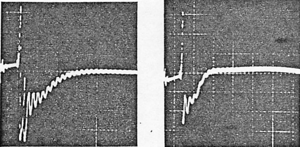
Fig. 1 (one feed) Fig. 2 (two feed) Transient phase shift during build up time. vertical: 18^\circ/\text{div} . horizontal: 20 \mu sec/div.
