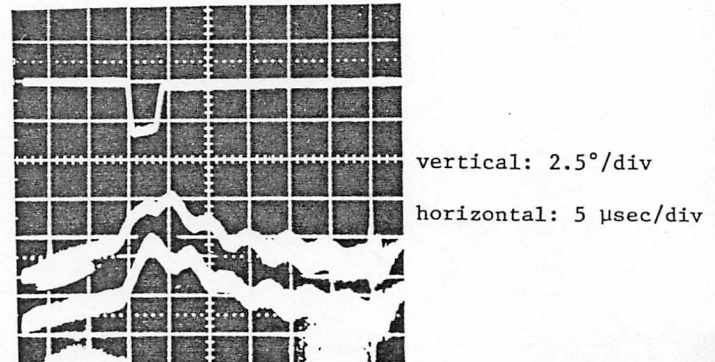
Fig. 6 Effect of TM011 mode on the phase shift. Wiggles of middle trace ( z=0.2L ) and those of lower trace ( z=0.9L ) are out of phase.
