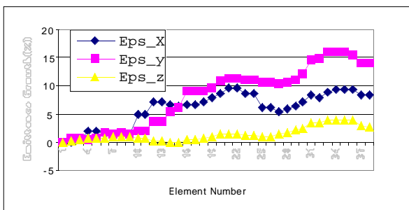
Figure 2. RMS Emittance growth along the beam line.
