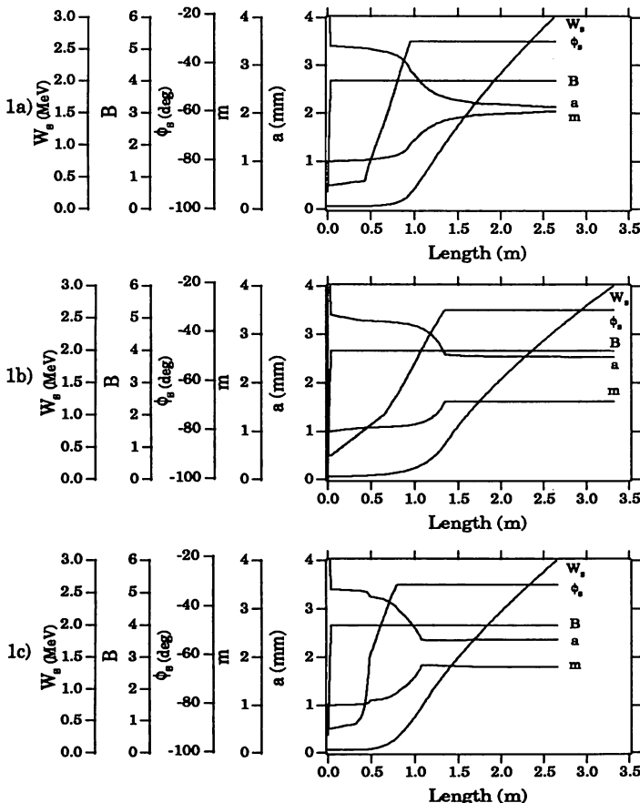
Fig. 1. The cell parameters of each design shown as functions of the longitudinal position: (a) KEKRFQ-D, (b) RFQUIK-D, (c) GENRFQ-D.
