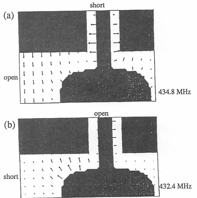
Fig. 12. Electric field patterns of the door-knob transition calculated with MAFIA.
