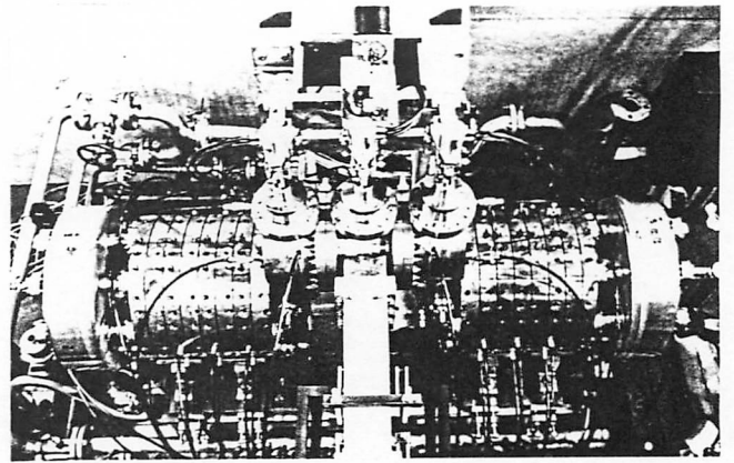
Fig.5 Photograph of the high-power ACS model.
