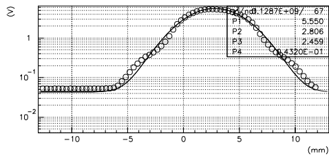
S03B:WSM01:X 調整前
