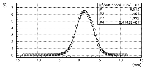
S03B:WSM01:X 調整前
