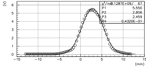
S03A:WSM01:X 調整前
