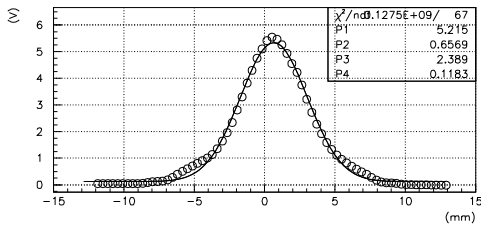
S03A:WSM01:Y 調整前
