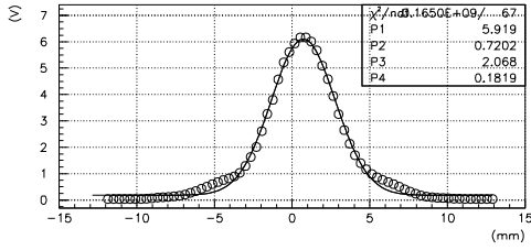
S02B:WSM01:Y 調整前
